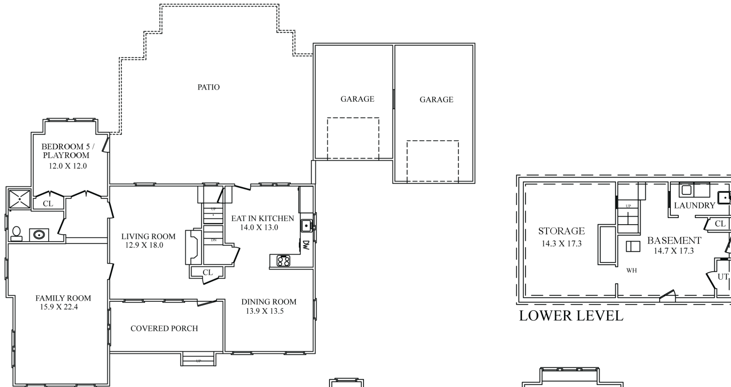
FIRST FLOOR
