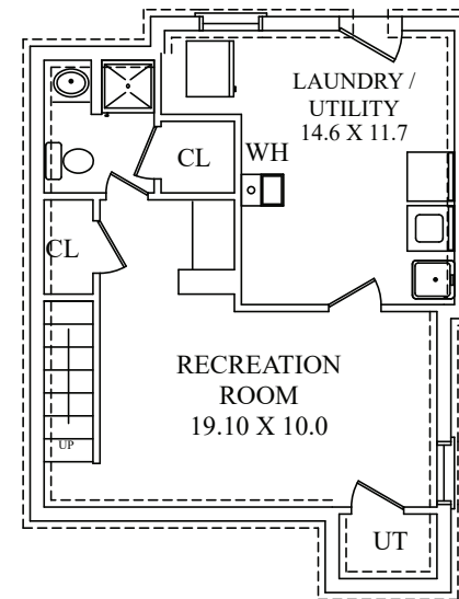
LOWER LEVEL
