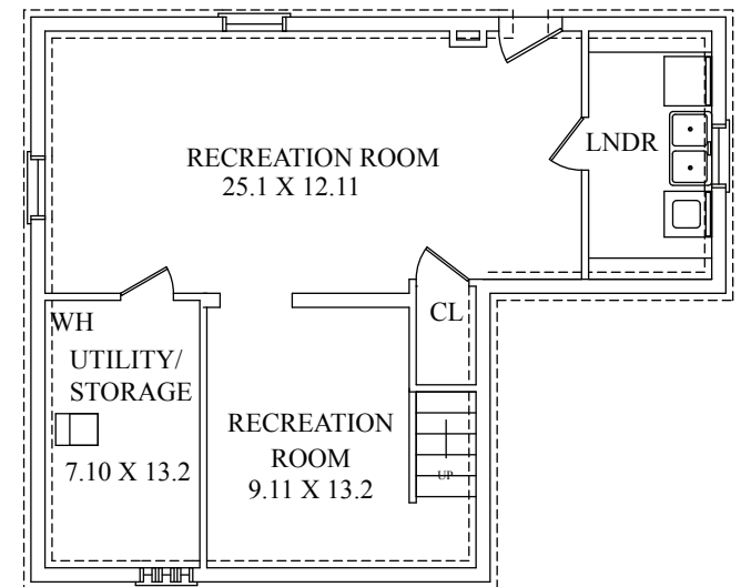
LOWER LEVEL
