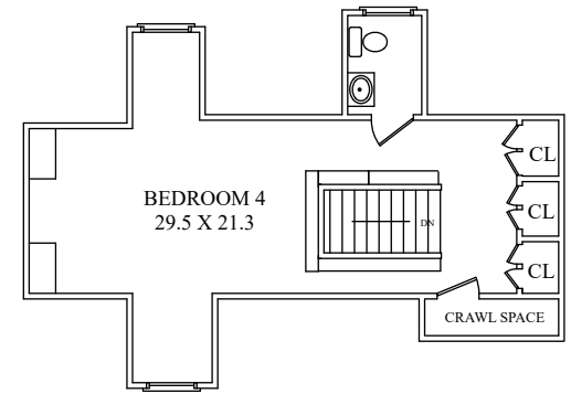
THIRD FLOOR
