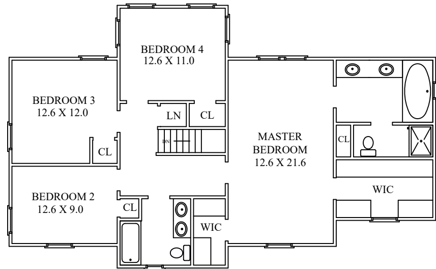
SECOND FLOOR
