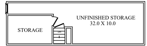
ATTIC
