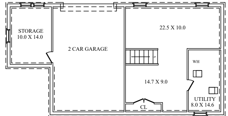
GROUND LEVEL
