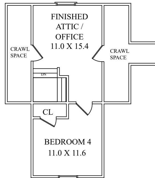
THIRD FLOOR
