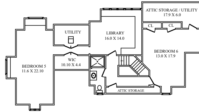
THIRD FLOOR
