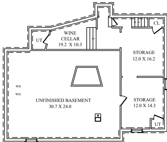
LOWER LEVEL
