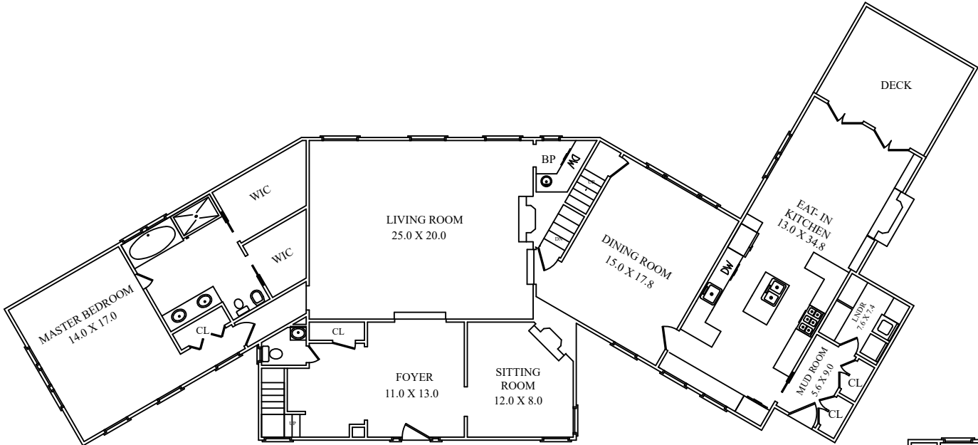
FIRST FLOOR
