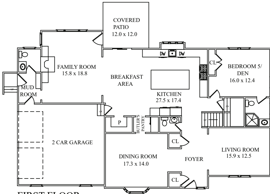
FIRST FLOOR
