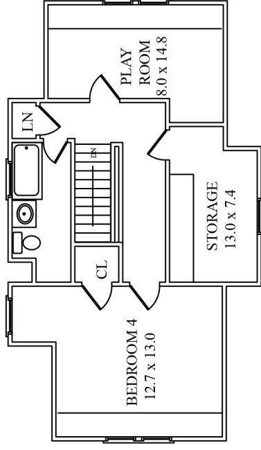
THIRD FLOOR
