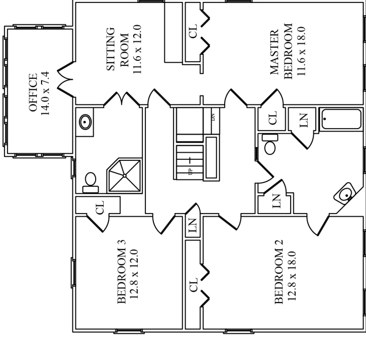
SECOND FLOOR
