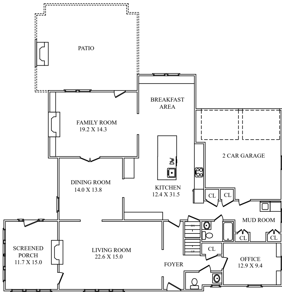
FIRST FLOOR
