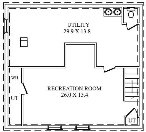
LOWER LEVEL
