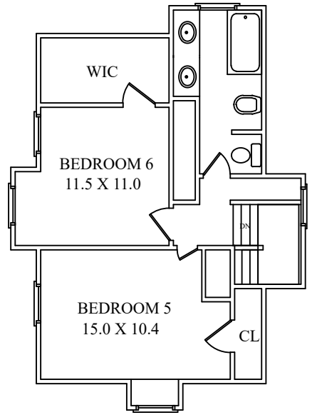
THIRD FLOOR
