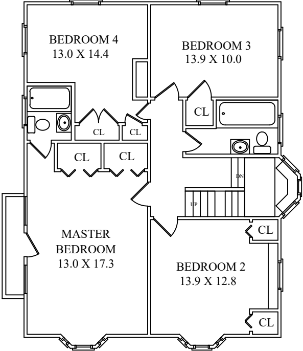
SECOND FLOOR
