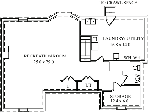
LOWER LEVEL
