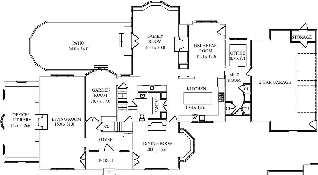
FIRST FLOOR
